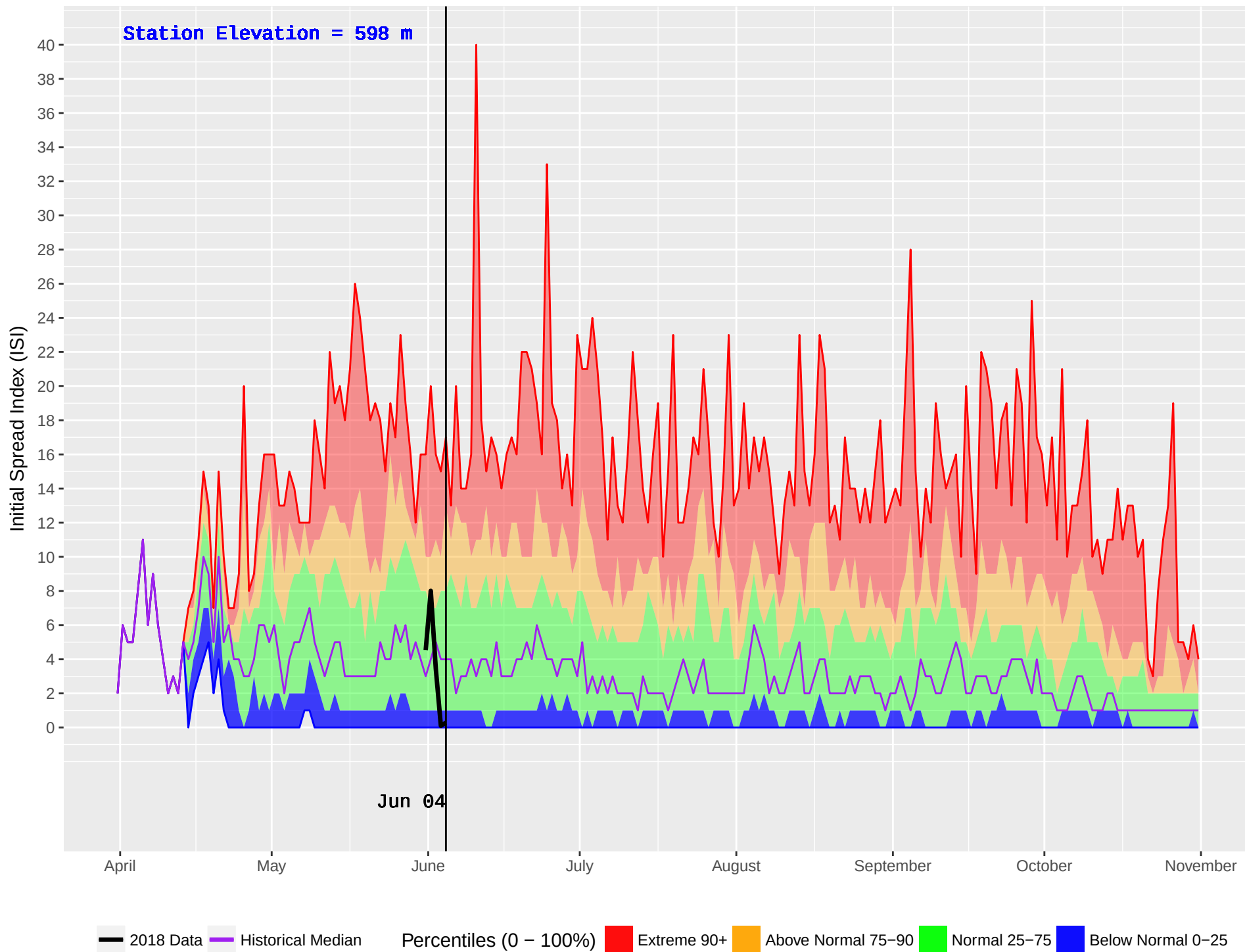
HELMUT (118) : Historical (1983–2016) and Current (2018) Noon Initial Spread Index (ISI)
